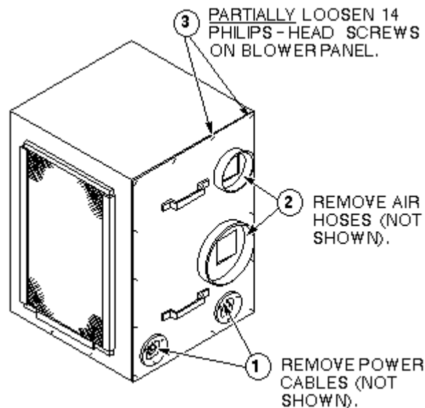
REMOVING BLOWER BOX MOTOR PANEL ILLUSTRATION 2-1
