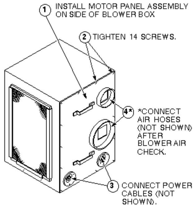
INSTALLING MOTOR PANEL ILLUSTRATION 2-5
