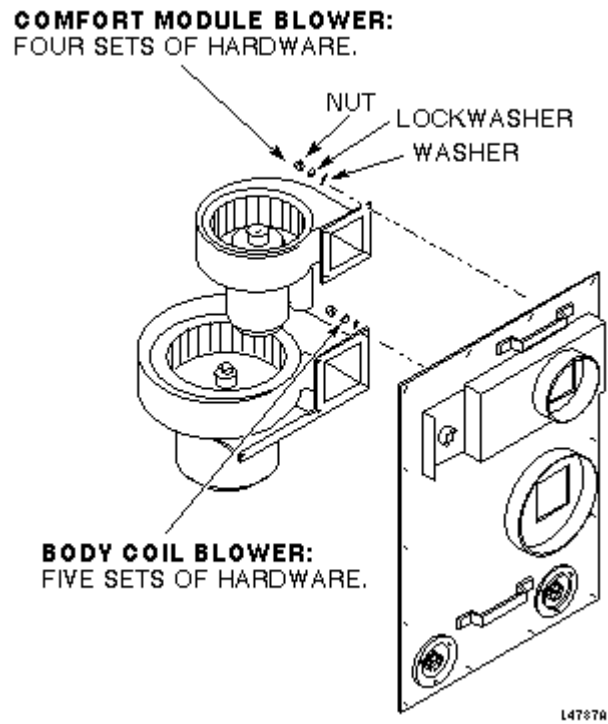
REMOVING/INSTALLING BLOWER MOTOR ILLUSTRATION 2-3
