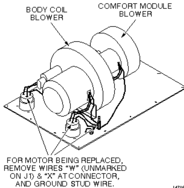
REMOVING BLOWER BOX MOTOR WIRING ILLUSTRATION 2-2
